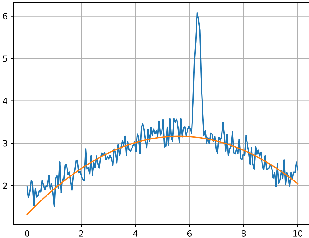
Continuum Fitting
