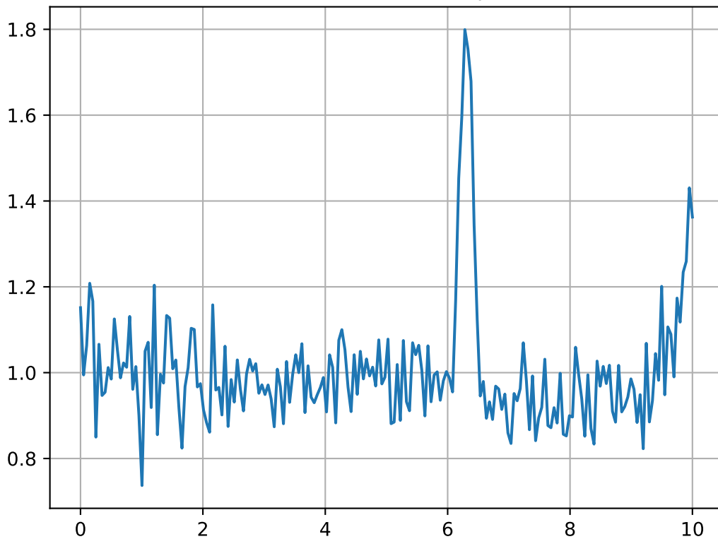
Continuum normalized spectrum
